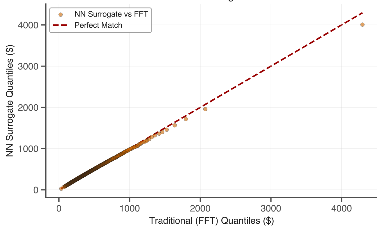
Q-Q Plot: NN Surrogate vs FFT
