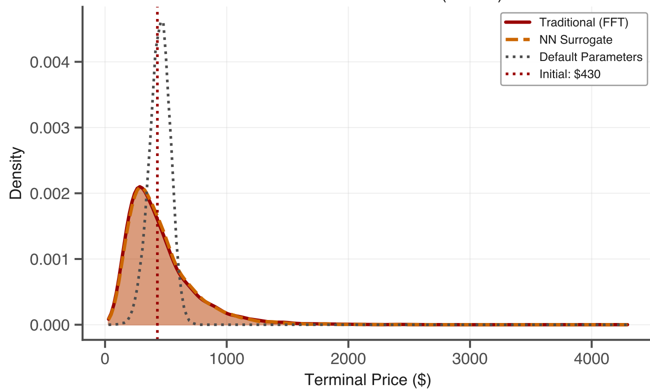
Terminal Price Distribution (1 Year)
