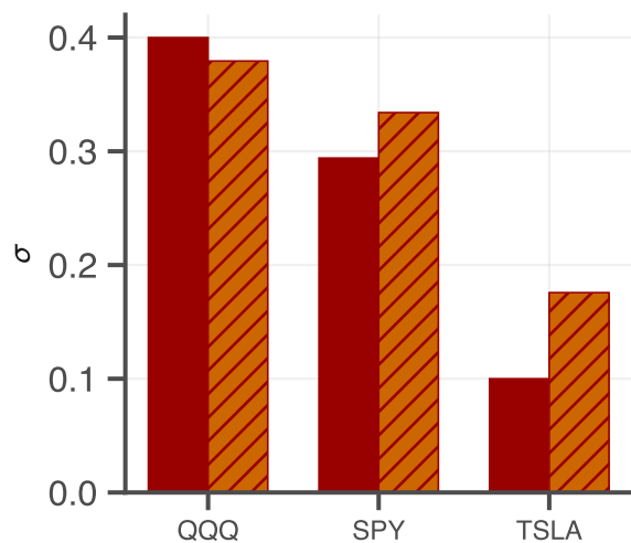
Vol of Vol
