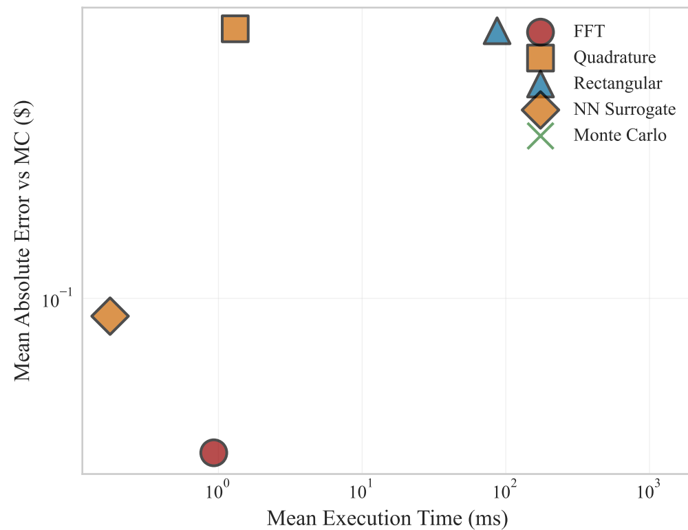
(a) Accuracy vs Speed Trade-off
