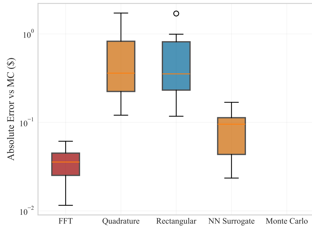
(b) Pricing Error Distribution
