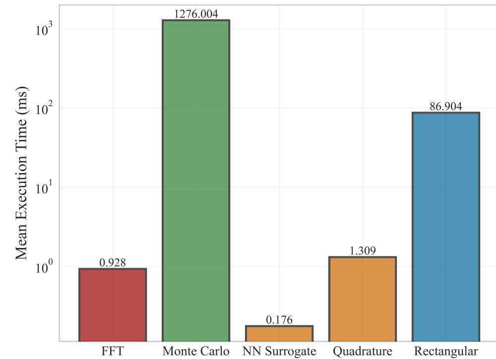
(c) Execution Time Comparison
