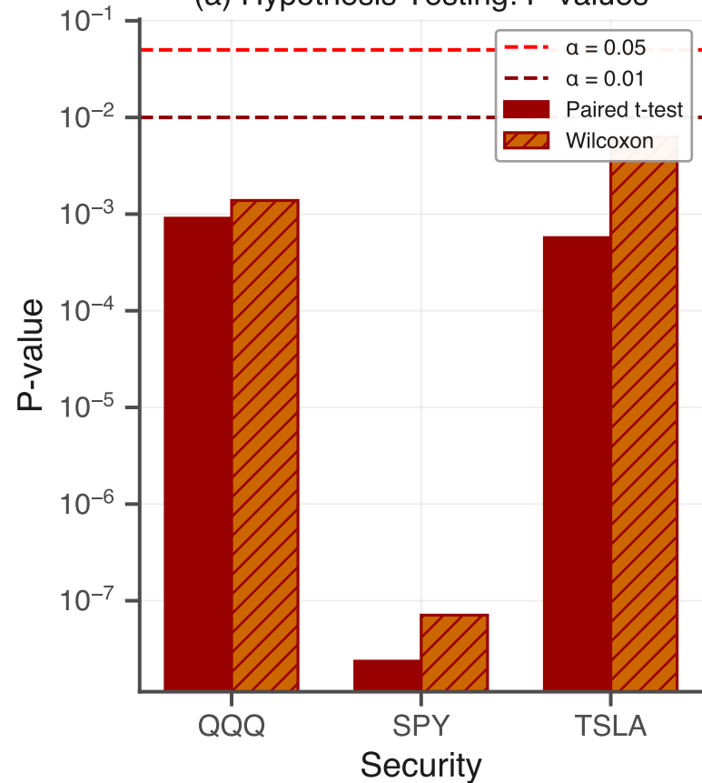
(a) Hypothesis Testing: P-values
