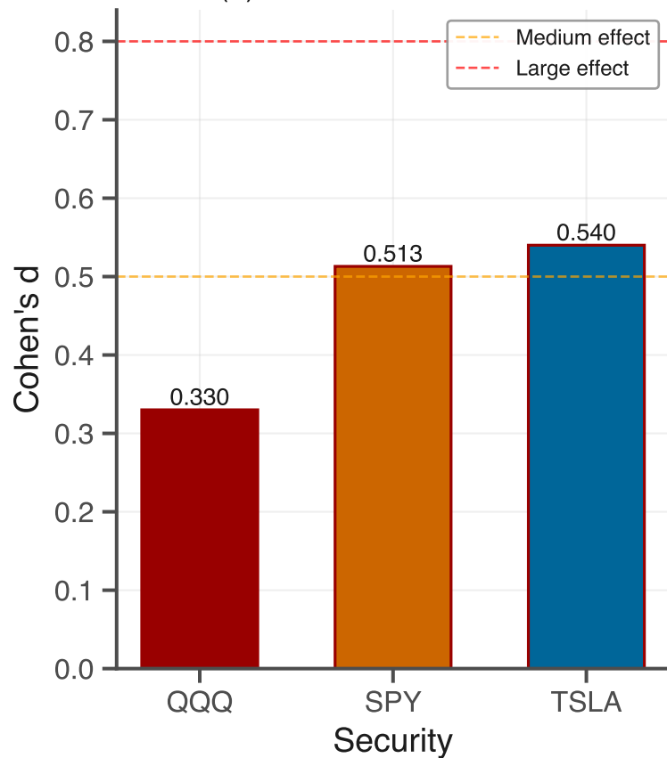
(b) Effect Size: Cohen's d
