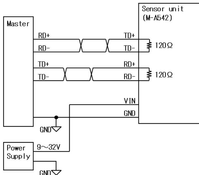
Figure 4.1 Connection Example
