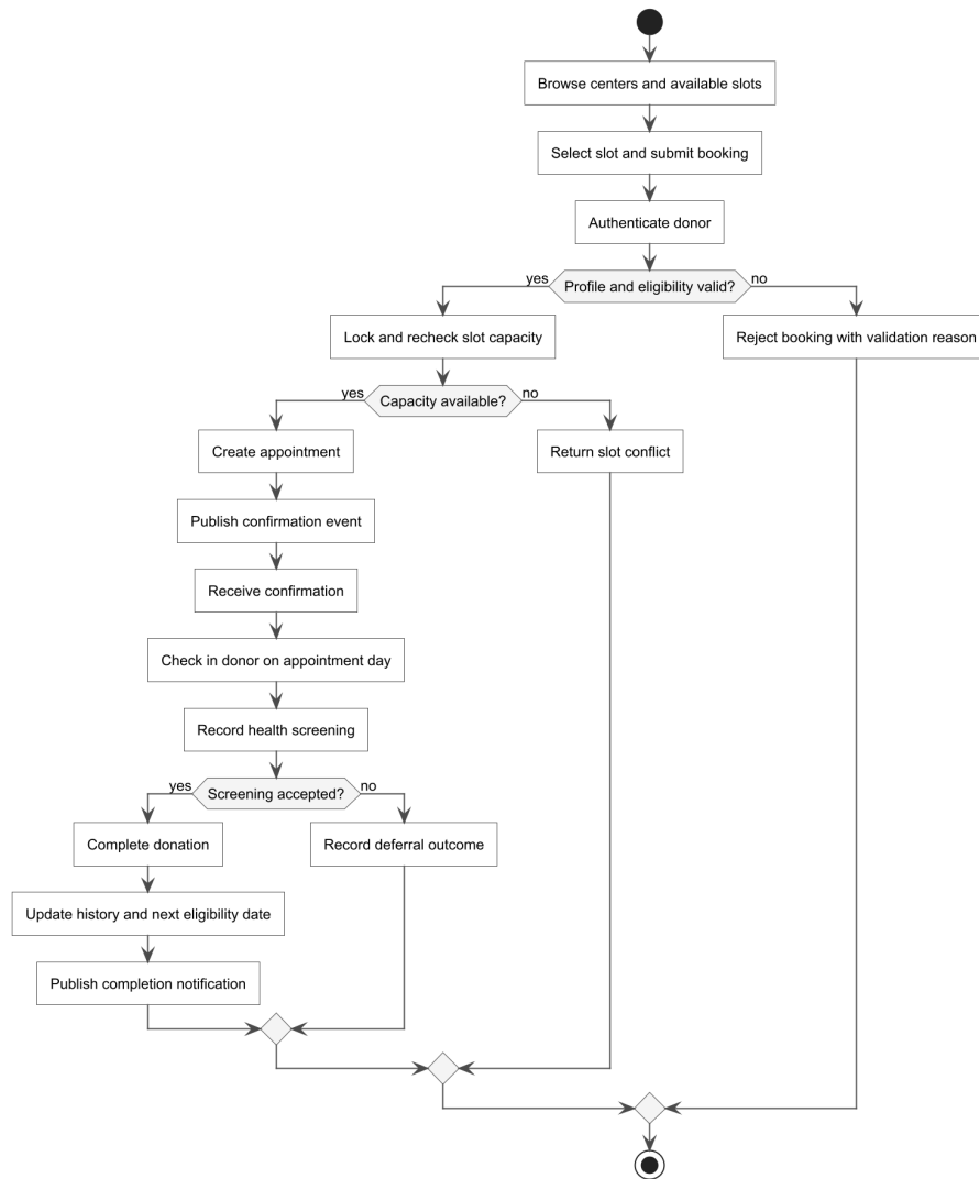
Figure 4.6: Appointment booking and donation activity diagram
