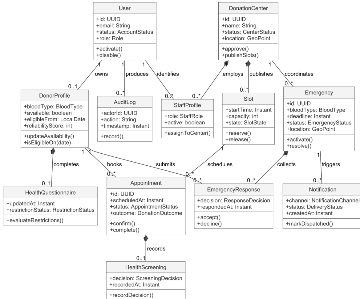
Figure 4.2: Global Qatra domain class diagram
