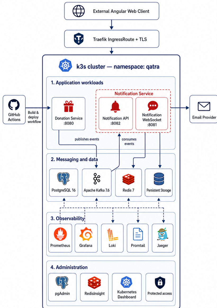
Figure 4.7: Verified physical k3s deployment in the single qatra namespace
