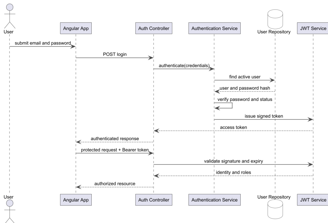
Figure 4.3: Authentication and protected request sequence Source: author; derived from the implemented Qatra system.
