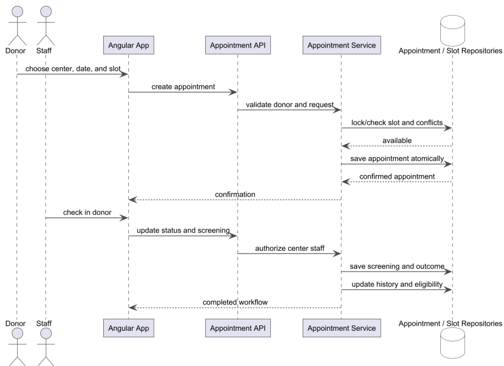
Figure 4.5: Appointment booking, check-in, screening, and completion sequence Source: author; derived from the implemented Qatra system.
