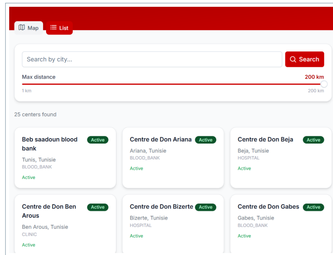
(b) Searchable center list
