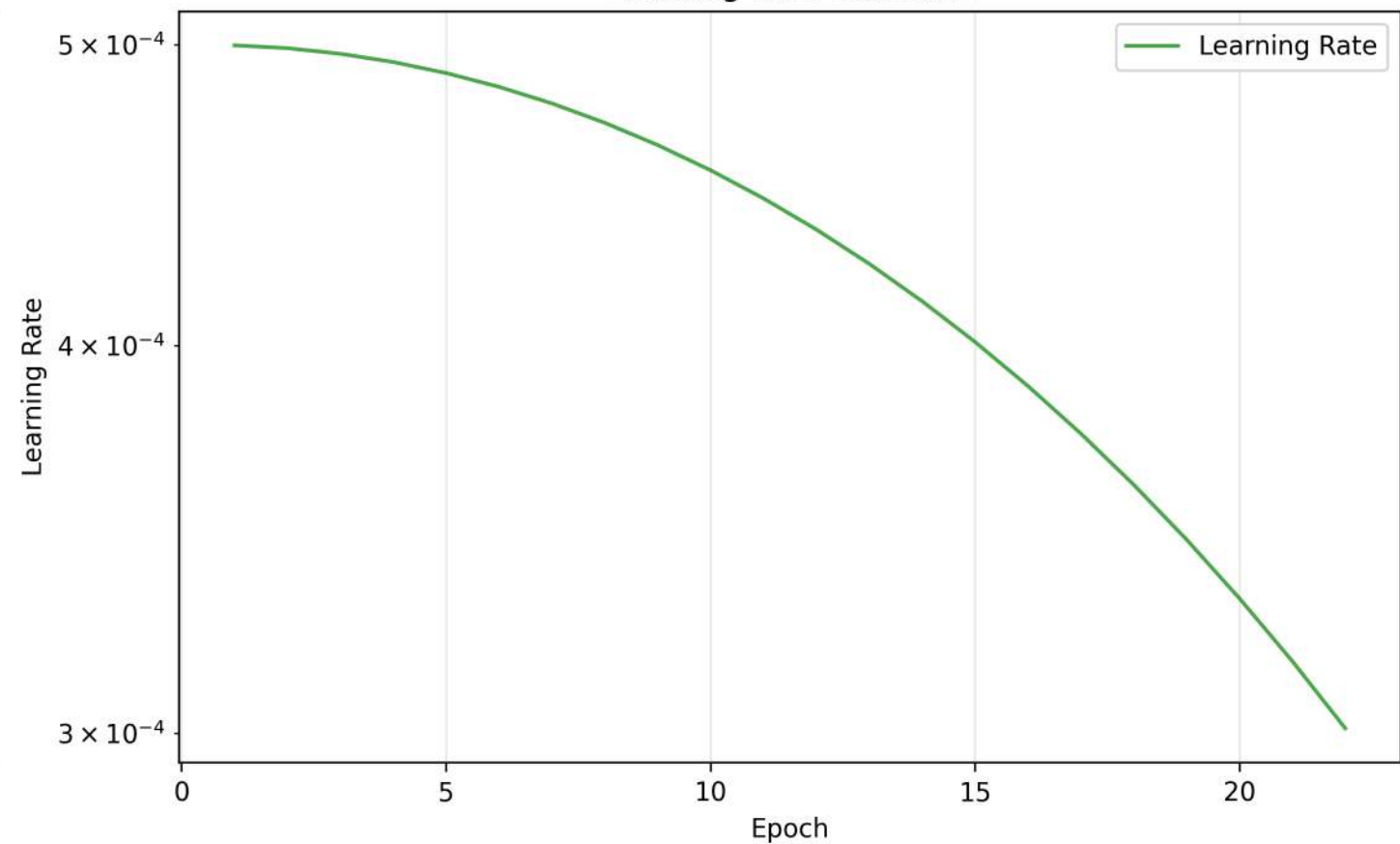
Learning Rate Schedule
