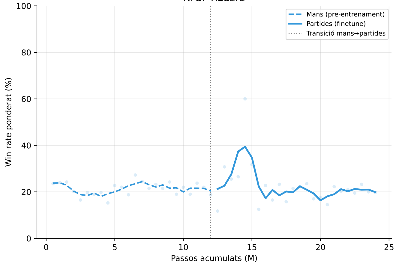
NFSP RLCard
