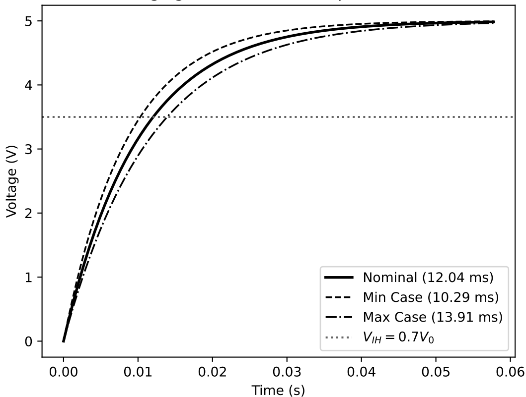
POR Charging Curves under Component Tolerances
