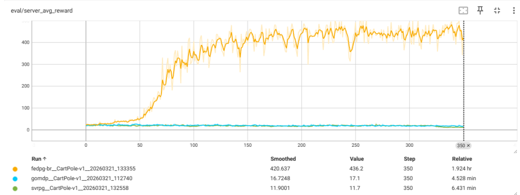
Figure 6.3: Convergence curves under Sign Flip attack (30% Byzantine). GOMDP and SVRPG collapse to near-zero reward while FedPG-BR maintains 420.
