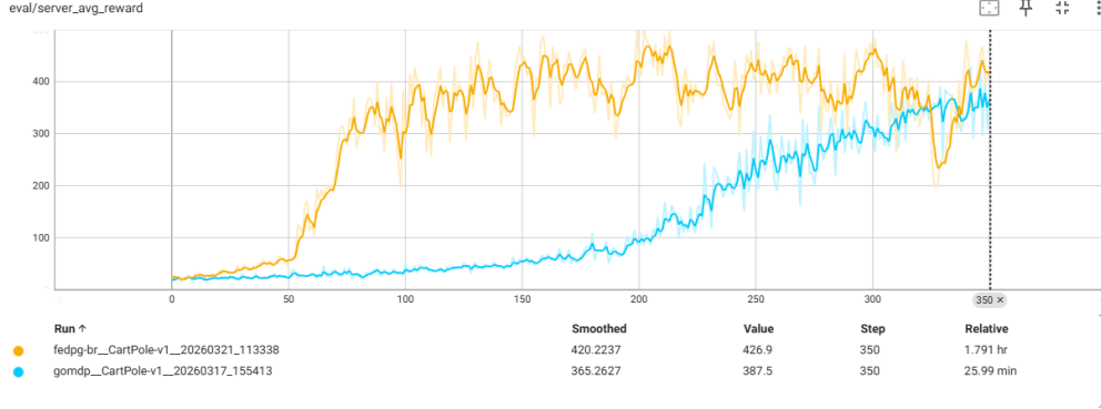
Figure 6.4: Convergence curves under Random Noise attack (30% Byzantine). GOMDP partially learns (365) as random gradients do not consistently corrupt the mean; FedPG-BR is unaffected (420).
