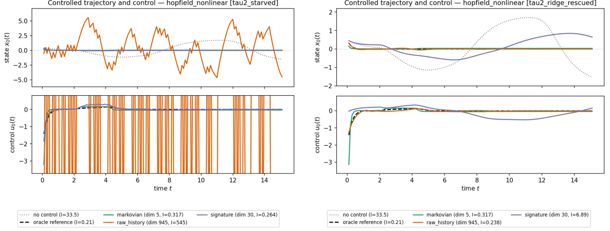
Figure 5: hopfield_nonlinear at \tau = 2 : the H_2 illusion and its cure. Left, the under-sampled fit ( n/\dim \varphi_H = 4.4 ): the history window (orange, dimension 945) diverges into a saturating bang-bang control ( J = 545 ) while the signature (purple) and oracle (dashed) track, so the signature appears preferable. Right, the same data with Tikhonov conditioning ( \lambda = 10^{-2} ): the history window is restored to J = 0.238 and tracks the oracle, while the identical ridge over-damps the signature ( J = 6.89 ). The cure is conditioning, not capacity (Finding 5.2).
