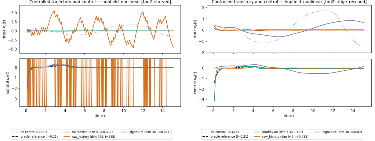
Figure 5: hopfield_nonlinear at \tau = 2 : the H_2 illusion and its cure. Left, the under-sampled fit ( n/\dim \phi_H = 4.4 ): the history window (orange, dimension 945) diverges into a saturating bang-bang control ( I = 545 ) while the signature (purple) and oracle (dashed) track, so the signature appears preferable. Right, the same data with Tikhonov conditioning ( \lambda = 10^{-2} ): the history window is restored to I = 0.238 and tracks the oracle, while the identical ridge over-damps the signature ( I = 6.89 ). The cure is conditioning, not capacity (Finding 5.2).
