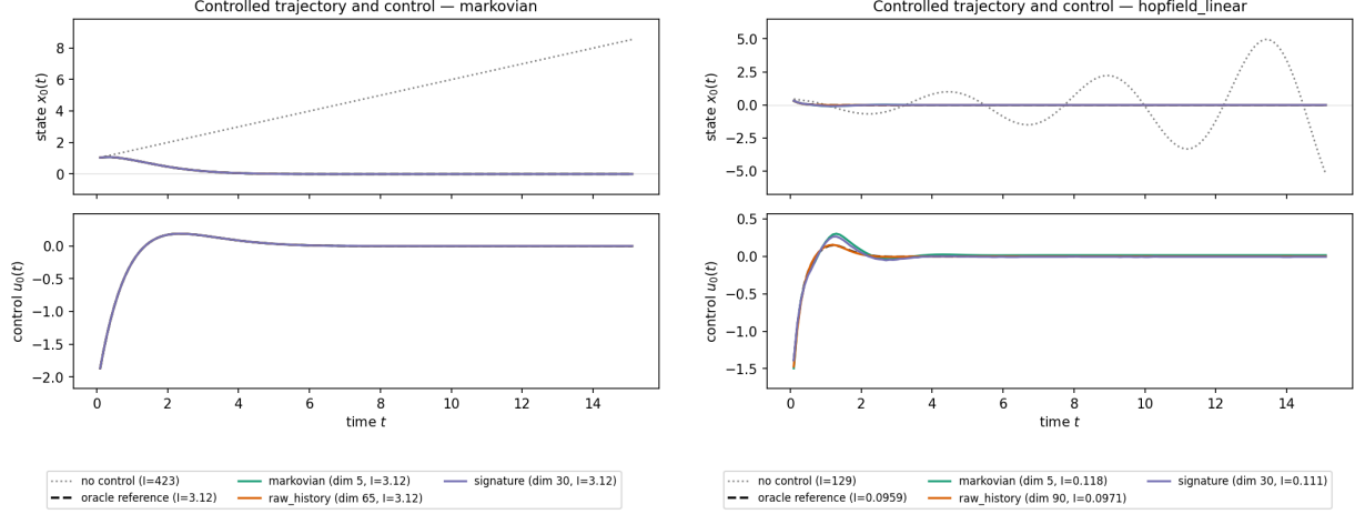
Figure 4: Left, markovian negative control: the three critics coincide (history irrelevant). Right, hopfield_linear : H_1 holds (history window below markovian), H_2 fails (signature above history window) — the provable-negative linear-in-delay arm.
