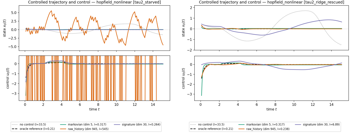
Figure 5: hopfield_nonlinear at \tau = 2 : the H_2 illusion and its cure. Left, the starved fit ( n/\dim \phi_H = 4.4 ): the history window (orange, dimension 945) diverges into a saturating bang-bang control ( I = 545 ) while the signature (purple) and oracle (dashed) track, so the signature appears to win. Right, the same data with Tikhonov conditioning ( \lambda = 10^{-2} ): the history window is restored to I = 0.238 and tracks the oracle, while the identical ridge over-damps the signature ( I = 6.89 ). The cure is conditioning, not capacity (Finding 5.2).
