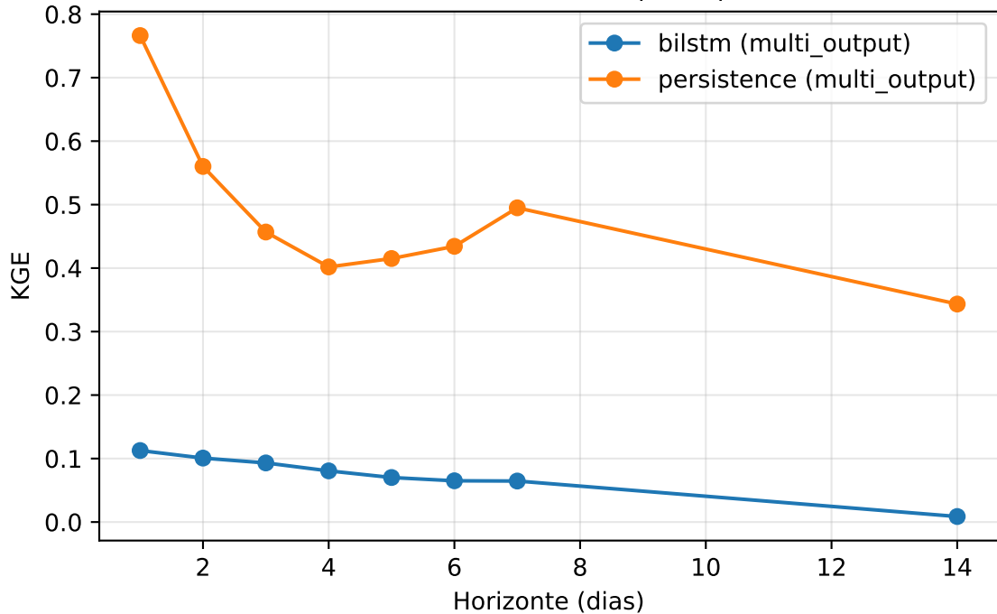
KGE vs. horizonte (TEST)
