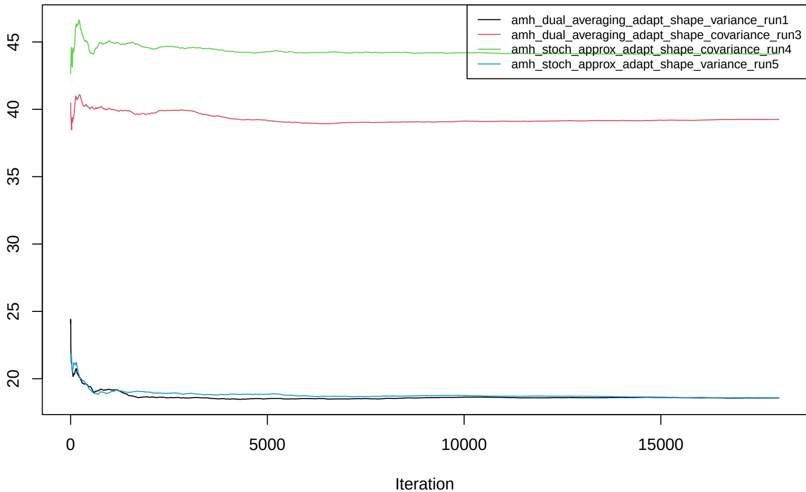
Running MSE of mean
