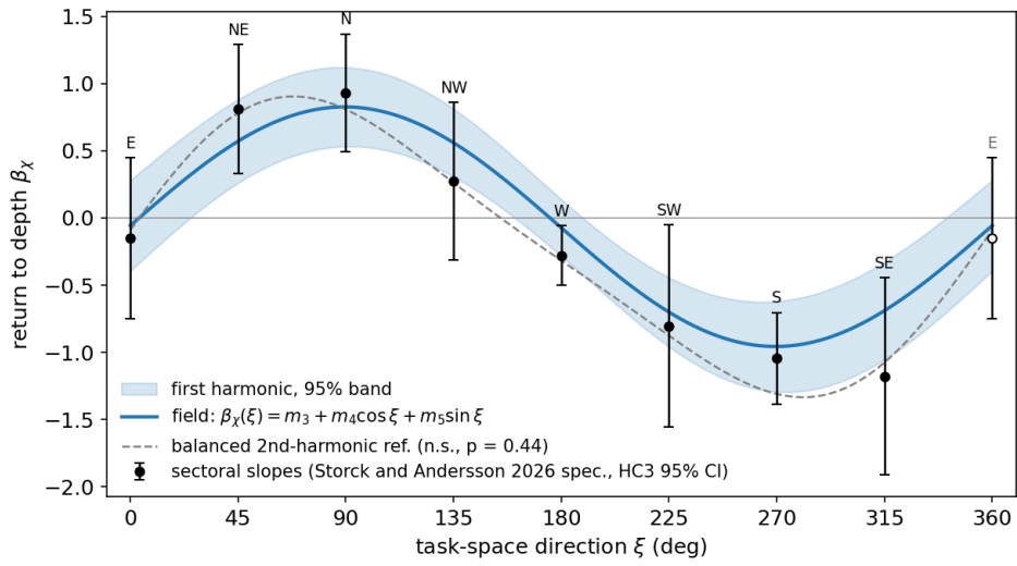
Figure 4: Directional return to depth, re-estimated on frozen inputs and compared to Storck and Andersson (2026).
