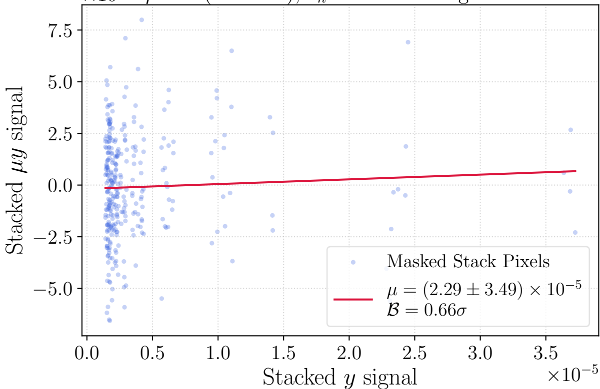
T-T Plot for \mu extraction, N = 10^3 , 200 iterations, PICO-like, \times 10^{-9} \mu = 0 (null test), s_n = \text{PICO} configuration
