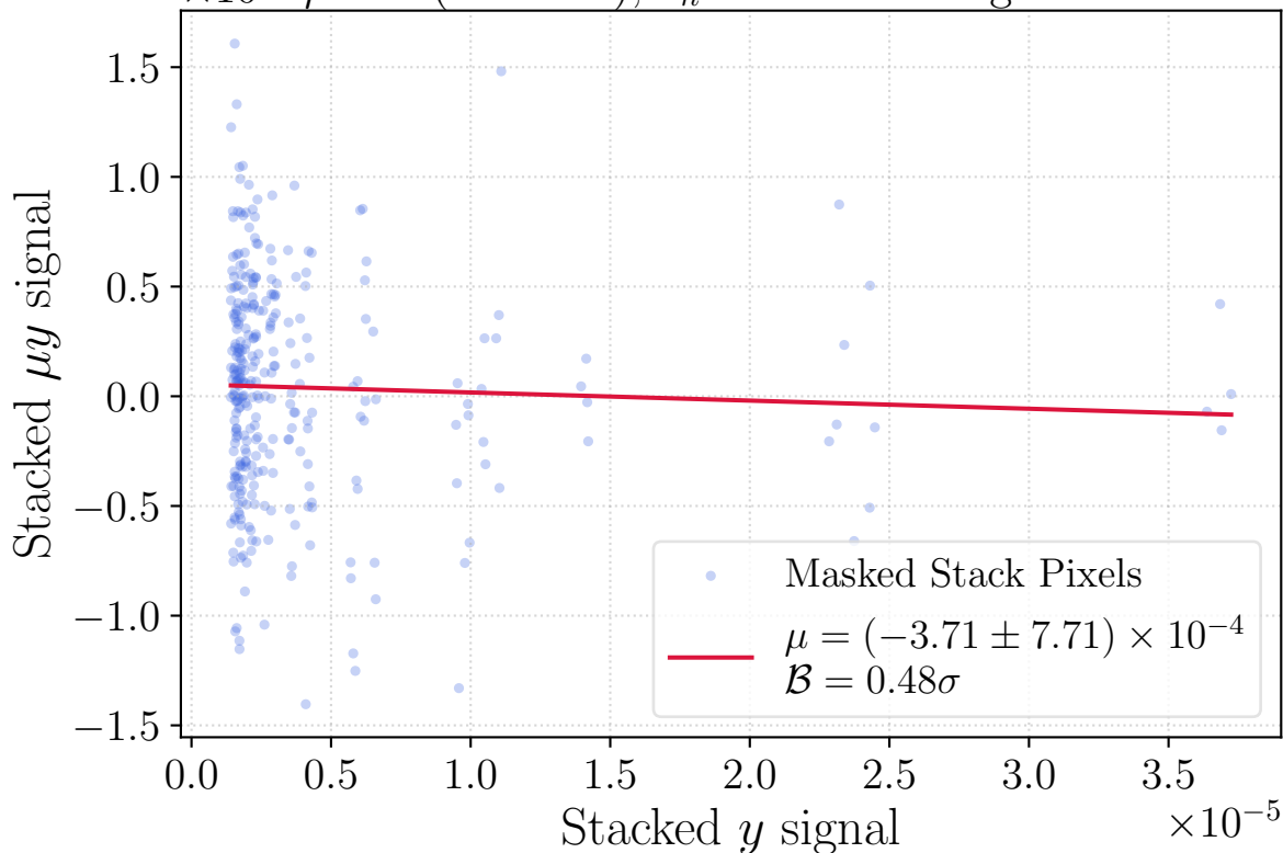
T-T Plot for \mu extraction, N = 10^3 , 200 iterations, PICO-like, \times 10^{-7} \mu = 0 (null test), s_n = \text{PICO} configuration
