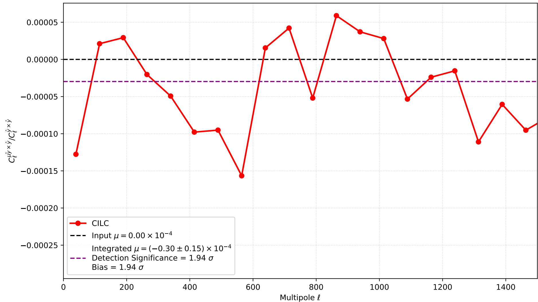
Binned spectral ratio for \mu extraction, \mu = 0\text{e}+00 , base sensitivity = 0.61 \mu\text{K}\cdot\text{arcmin}
