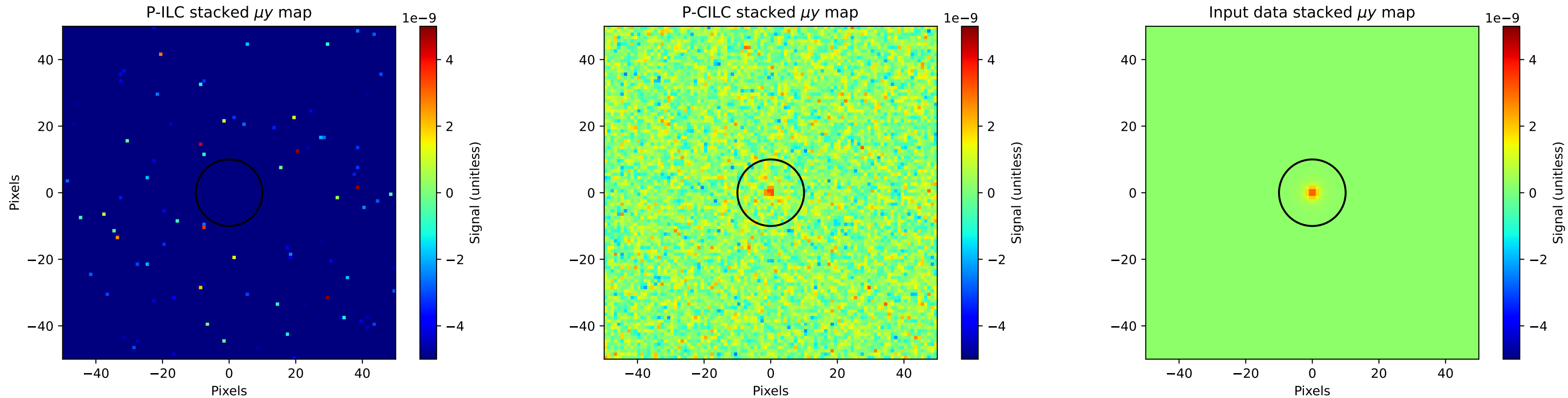
Comparison of \mu y map stacked patches of 1e+04 brightest clusters, \mu value = 2e-04 , base sensitivity = 0.20 \mu K \cdot \text{arcmin} , r = 10p
