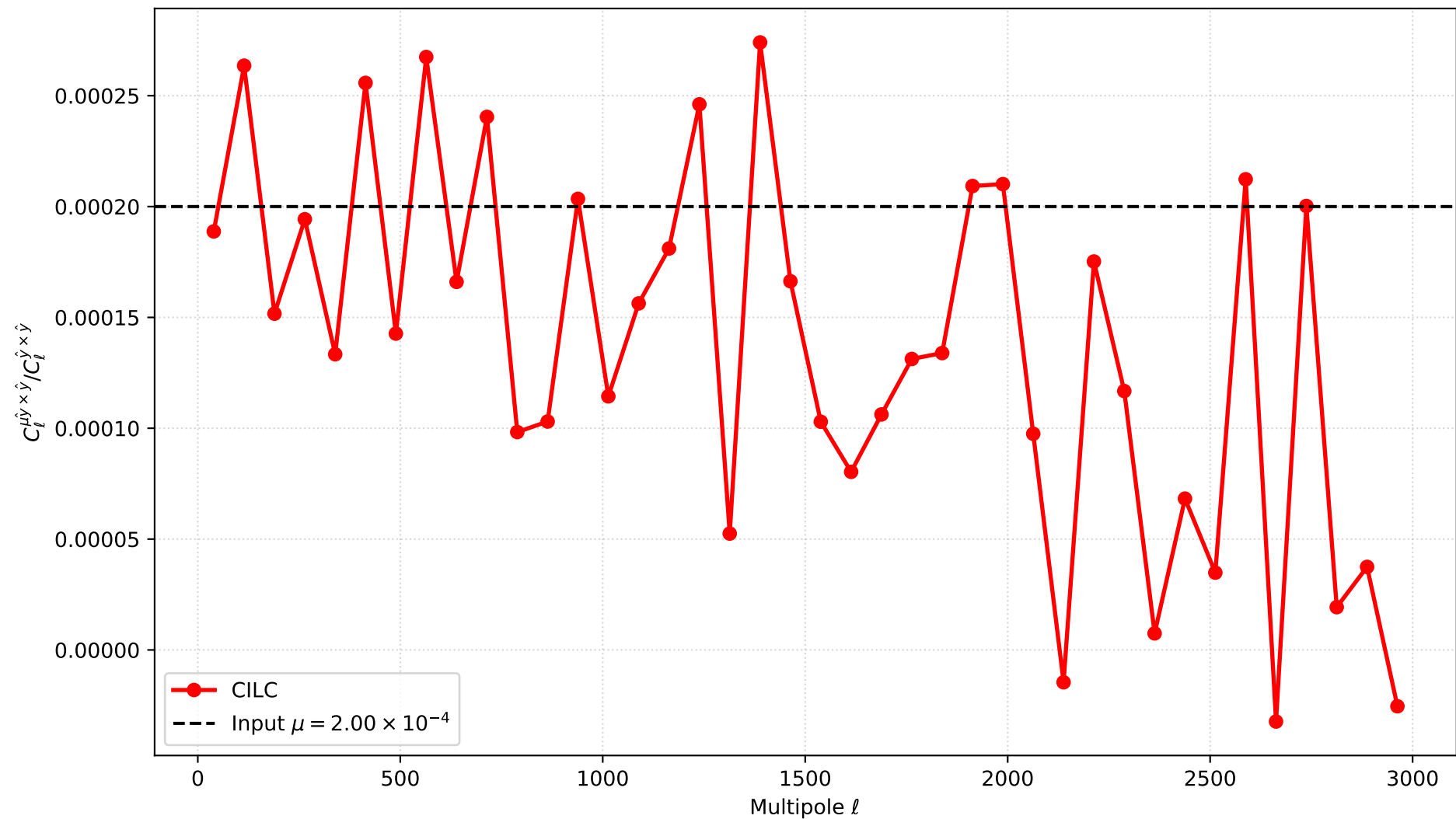
Binned spectral ratio for \mu extraction, \mu = 2\text{e-}04 , base sensitivity = 0.61 \mu\text{K}\cdot\text{arcmin}
