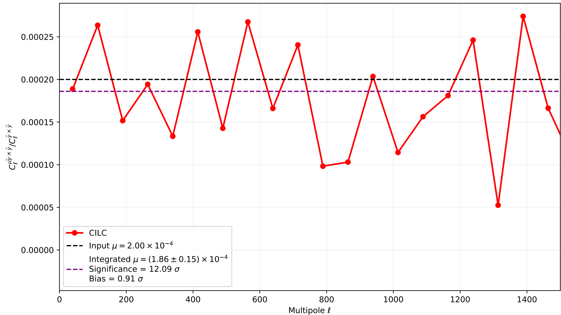
Binned spectral ratio for \mu extraction, \mu = 2\text{e-}04 , base sensitivity = 0.61 \mu\text{K}\cdot\text{arcmin}
