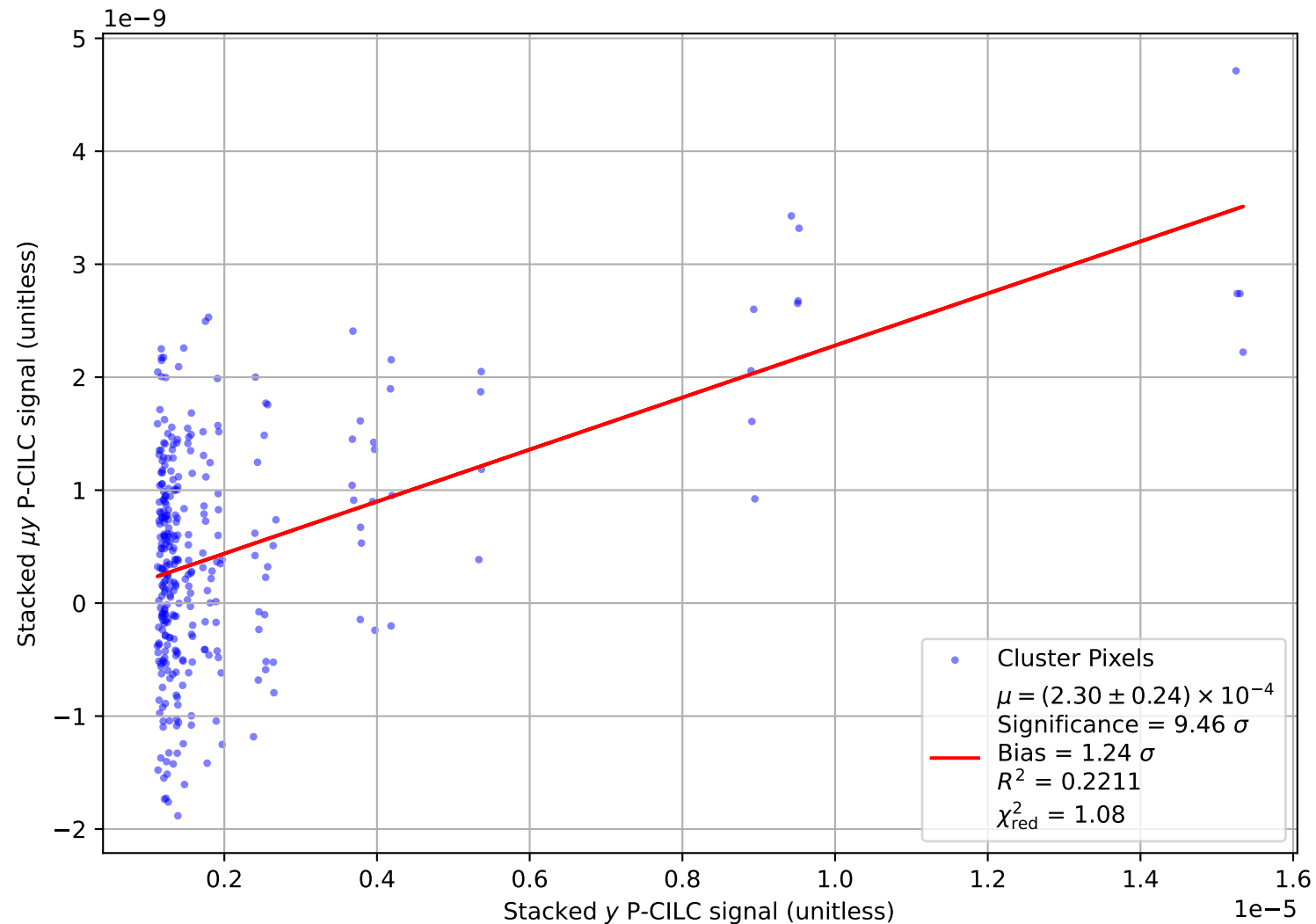
T-T Plot: P-CILC \mu y Vs. P-CILC y, \mu = 2\text{e-}04 , base sensitivity = 0.61 \mu\text{K}\cdot\text{arcmin} , r \leq 10 pixels, PICO
