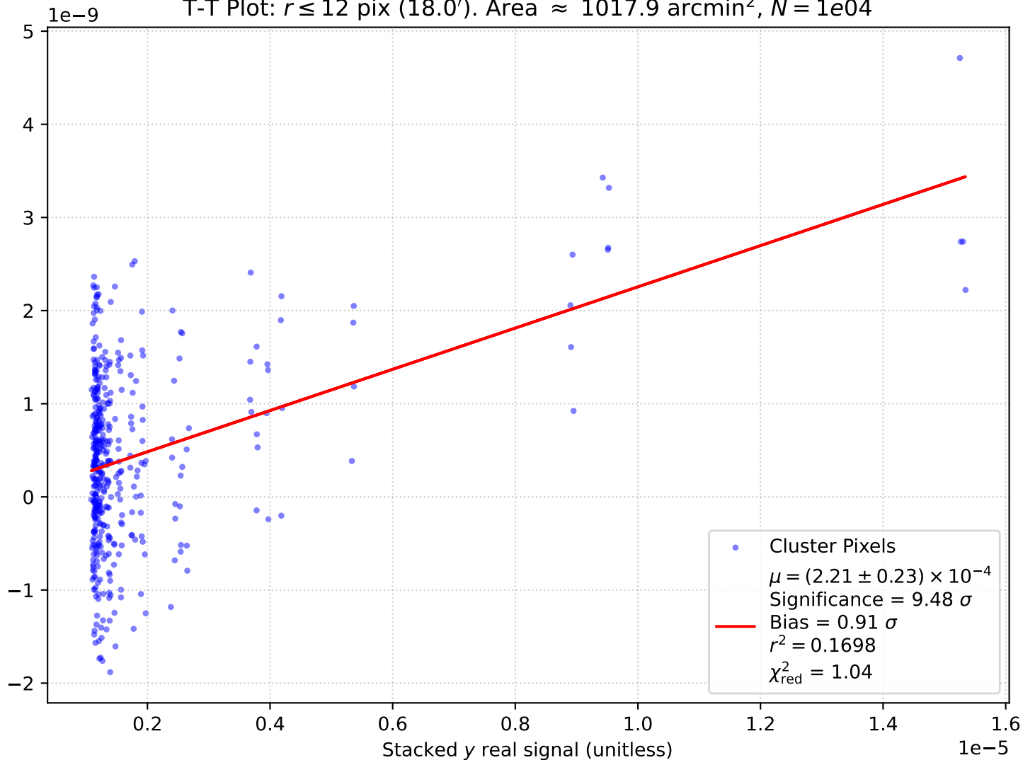
T-T Plot: r \leq 12 pix (18.0'). Area \approx 1017.9 arcmin 2 , N = 1e04
