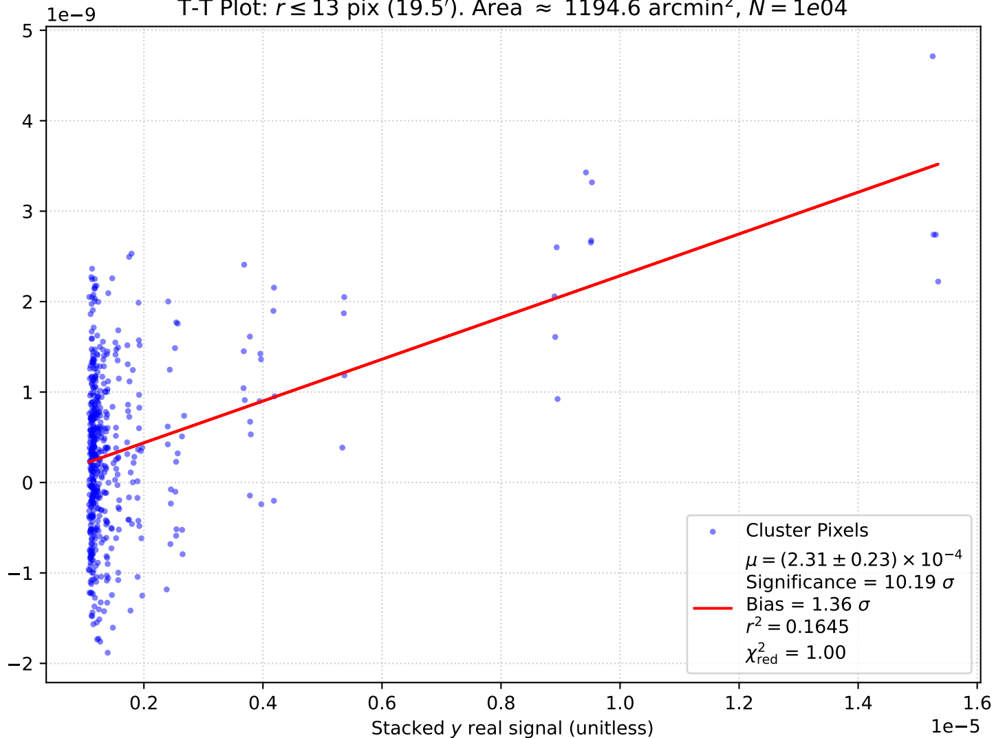
T-T Plot: r \leq 13 pix (19.5'). Area \approx 1194.6 arcmin 2 , N = 1e04
