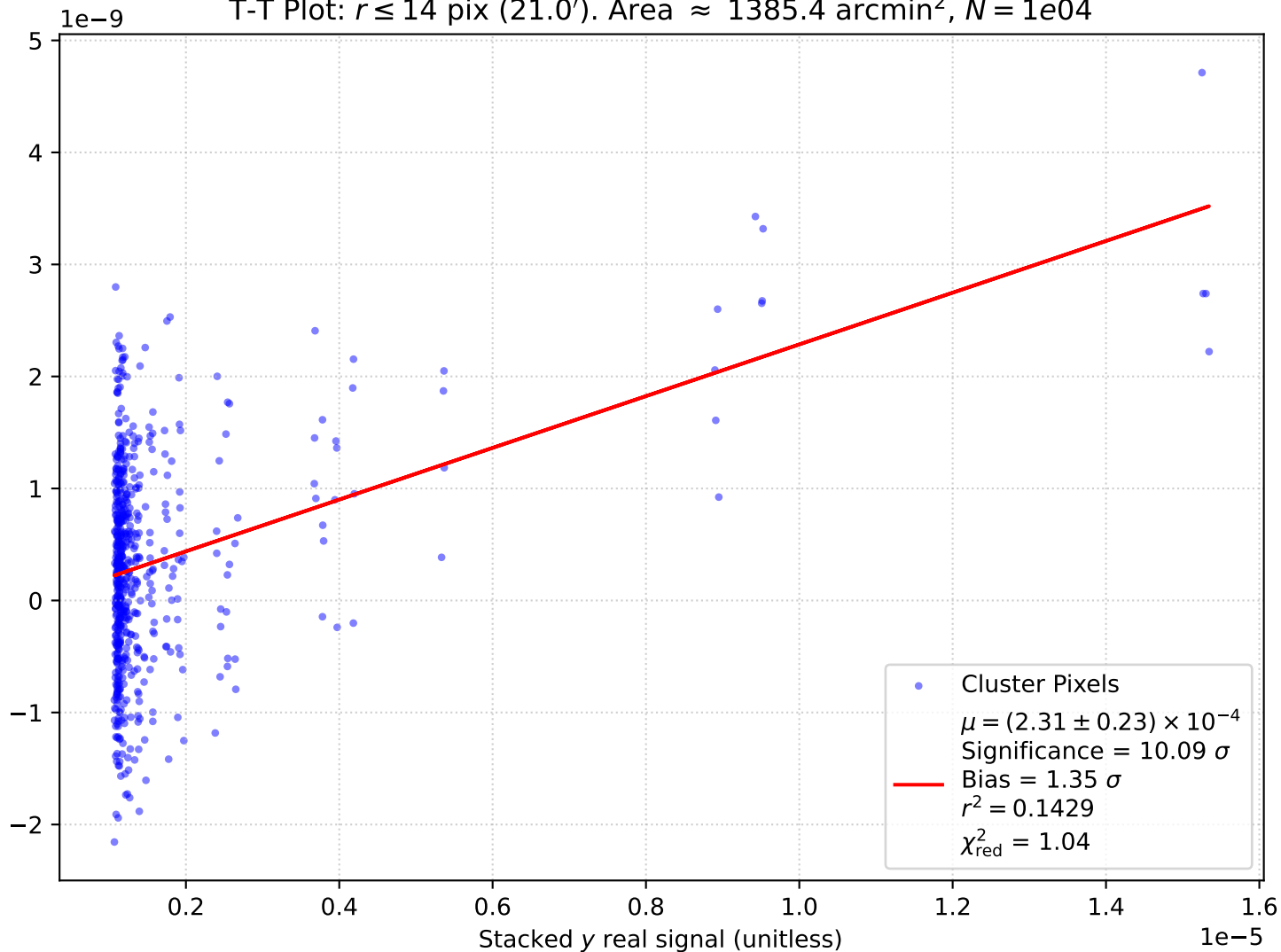
T-T Plot: r \leq 14 pix (21.0'). Area \approx 1385.4 arcmin 2 , N = 1e04
