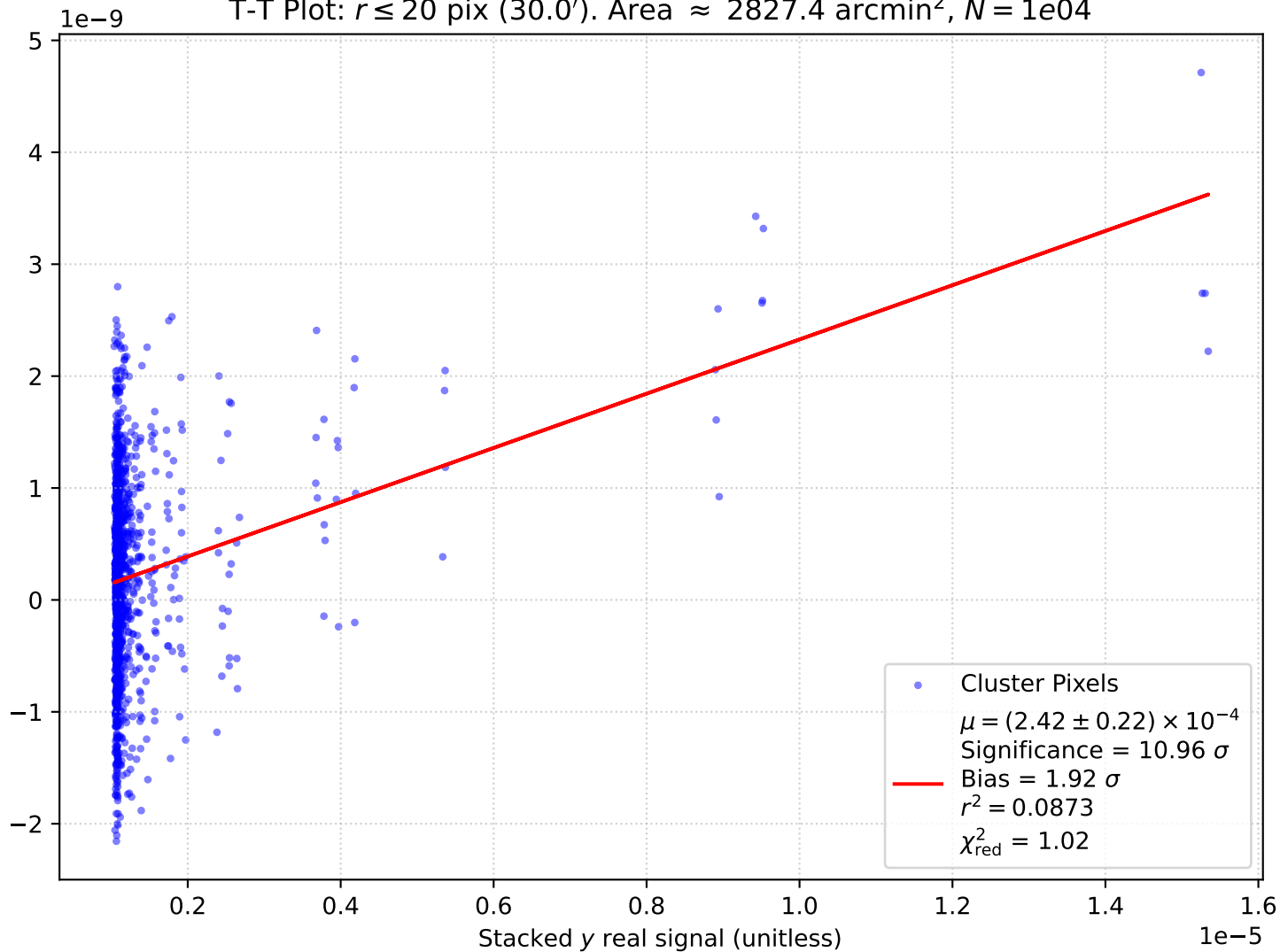
T-T Plot: r \leq 20 pix (30.0'). Area \approx 2827.4 arcmin 2 , N = 1e04
