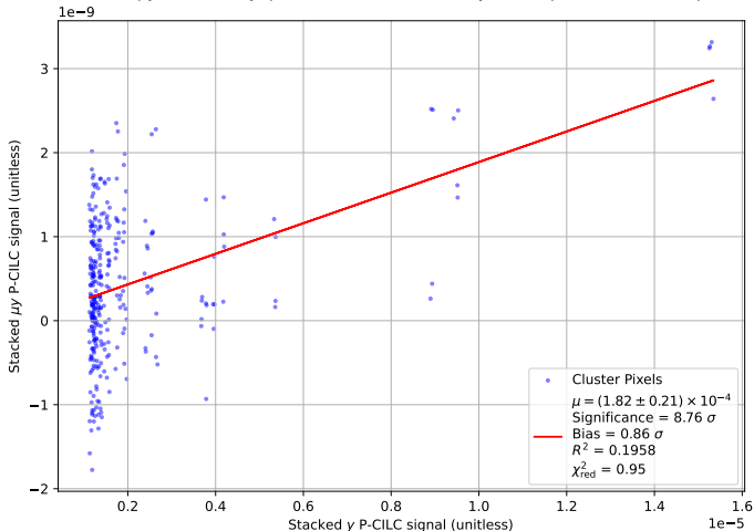
T-T Plot: P-CILC \mu y Vs. P-CILC y , \mu = 2\text{e-}04 , base sensitivity = 0.20 \mu K \cdot \text{arcmin} , r \leq 10 pixels, PICO
