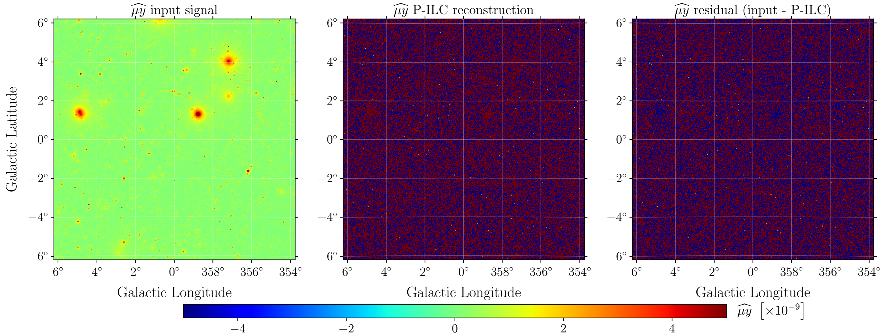
Zoomed input map and P-ILC reconstructed and residual \widehat{\mu y} maps, \mu = 2 \times 10^{-4} , PICO configuration
