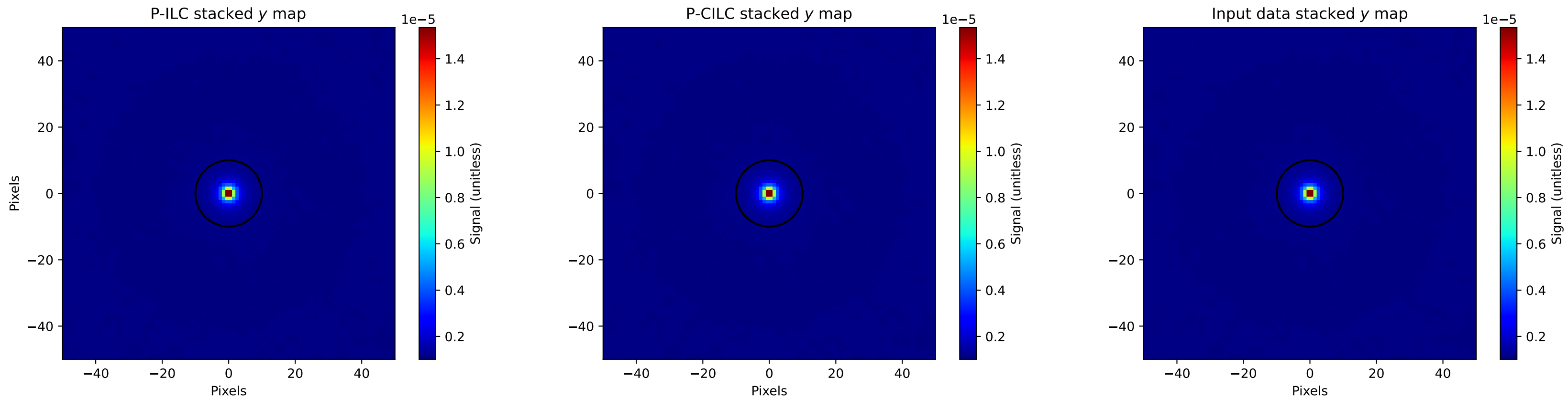
Comparison of y map stacked patches of 1\text{e}+04 brightest clusters, \mu value = 0\text{e}+00 , base sensitivity = 0.20\ \mu\text{K}\cdot\text{arcmin} , r = 10\text{p}
