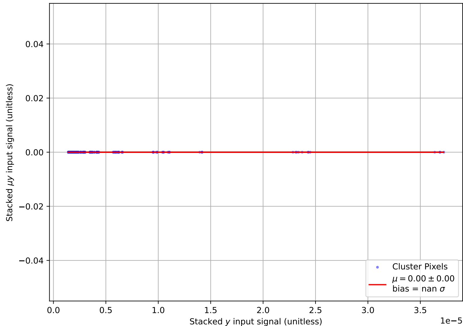
T-T Plot: input \mu y Vs. input y , \mu = 0\text{e}+00 , base sensitivity = 0.20 \mu\text{K}\cdot\text{arcmin} , r \leq 10 pixels
