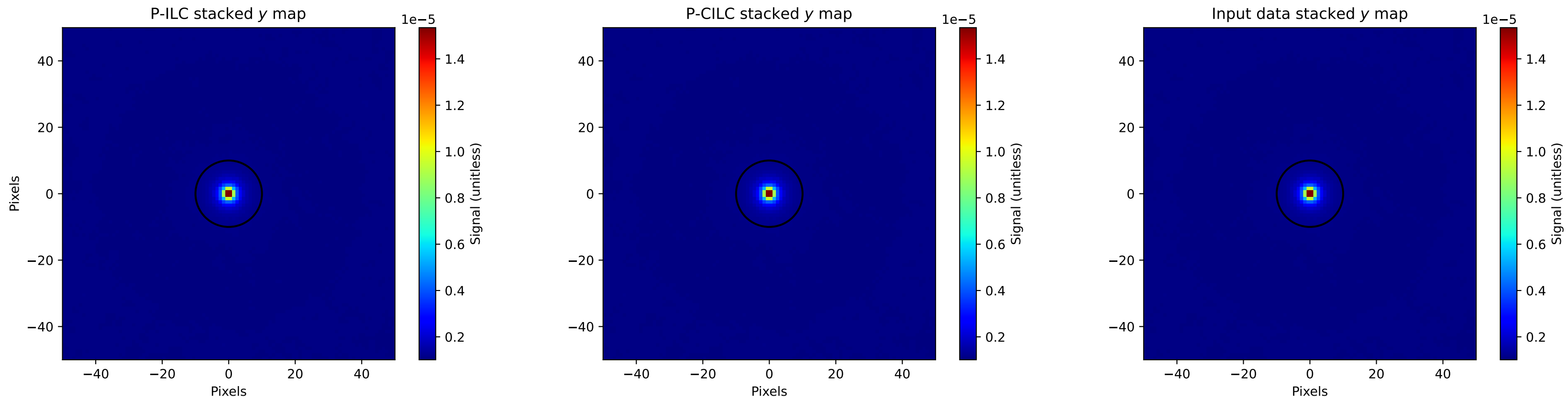
Comparison of y map stacked patches of 1\text{e}+04 brightest clusters, \mu value = 2\text{e}-05 , base sensitivity = 0.20\ \mu\text{K}\cdot\text{arcmin} , r = 10\text{p}
