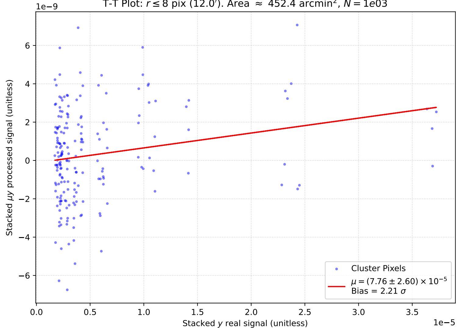
T-T Plot: r \leq 8 pix (12.0'). Area \approx 452.4 arcmin 2 , N = 1e03
