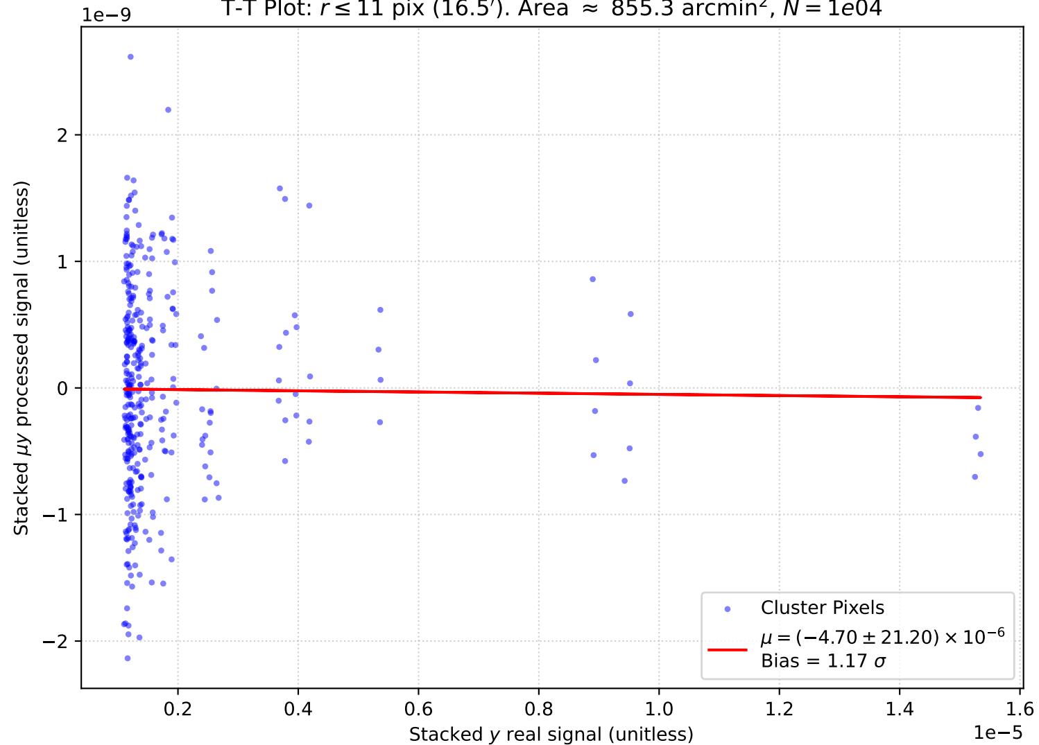
T-T Plot: r \leq 11 pix (16.5'). Area \approx 855.3 arcmin 2 , N = 1e04
