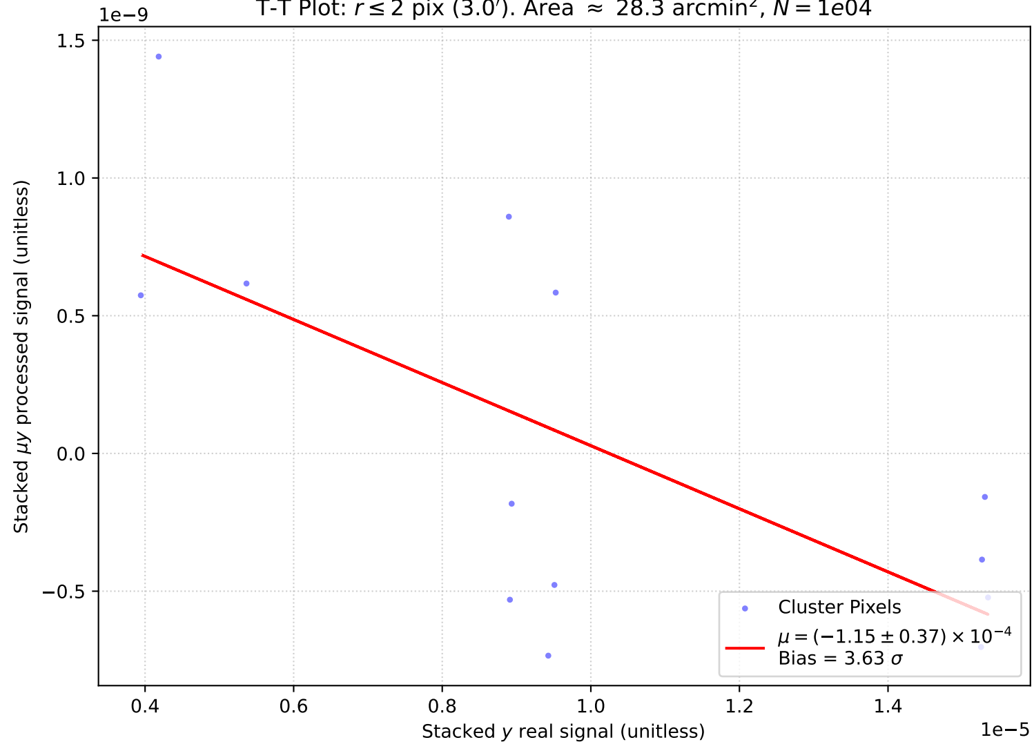
T-T Plot: r \leq 2 pix ( 3.0' ). Area \approx 28.3 arcmin 2 , N = 1e04
