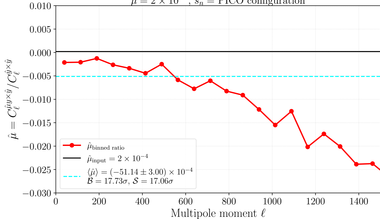
Binned spectral ratio for \mu extraction, PICO configuration, \mu = 2 \times 10^{-4} , s_n = \text{PICO configuration}
