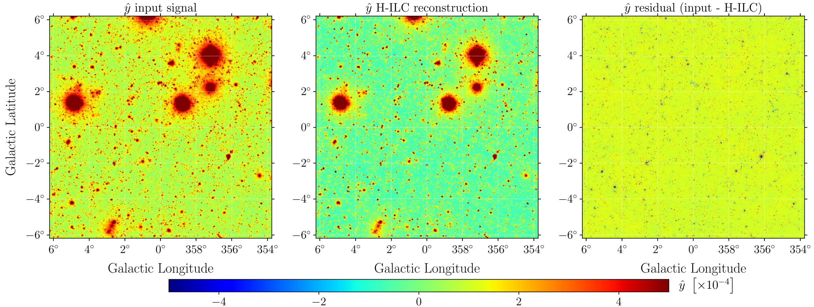
Zoomed input map and H-ILC reconstructed and residual \hat{y} maps, \mu = 2 \times 10^{-4} , PICO configuration
