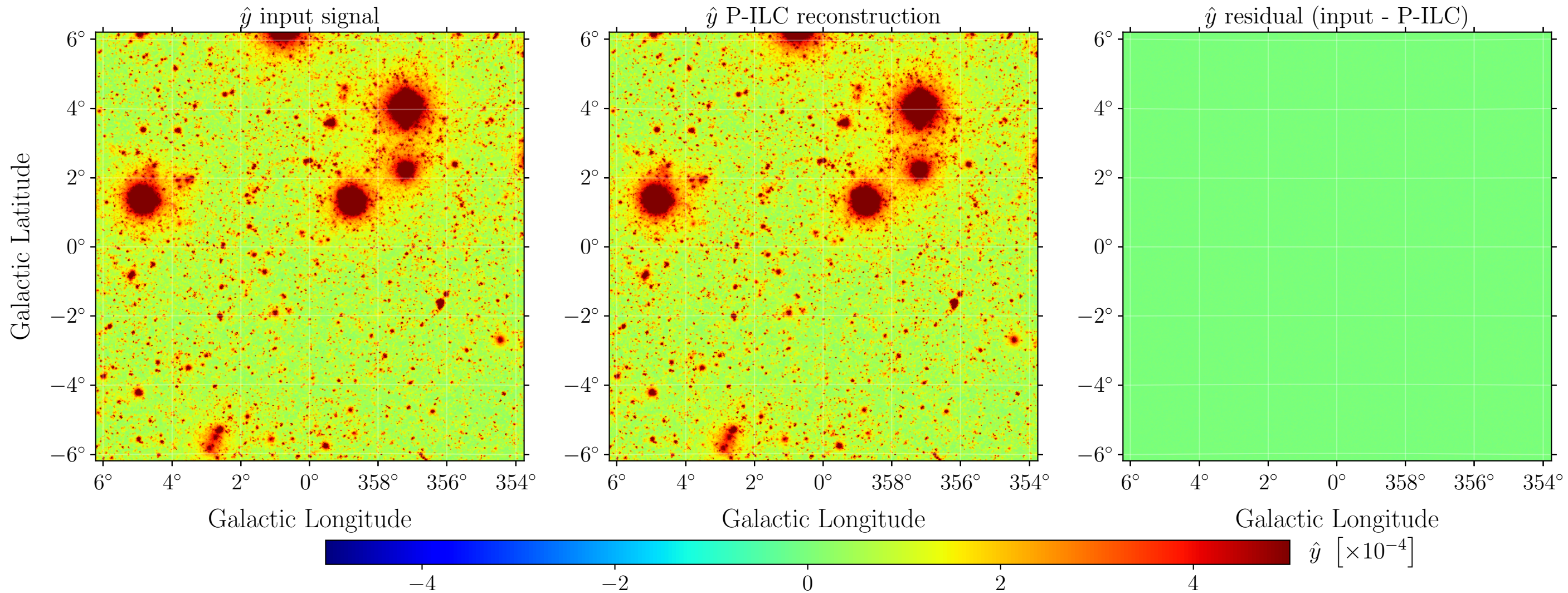
Zoomed input map and P-ILC reconstructed and residual \hat{y} maps, \mu = 2 \times 10^{-4} , PICO configuration
