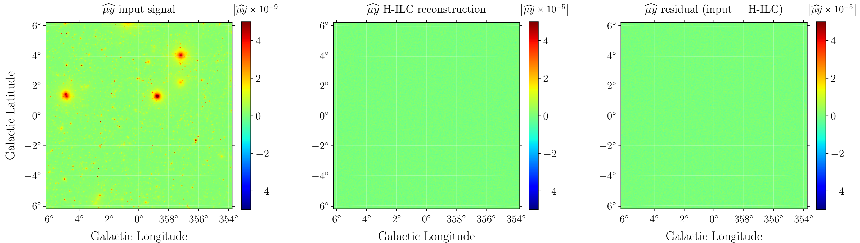
Zoomed input map and H-ILC reconstructed and residual \widehat{\mu y} maps, \mu = 2 \times 10^{-4} , PICO configuration
