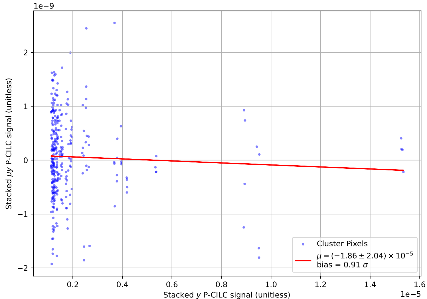
T-T Plot: P-CILC \mu y Vs. P-CILC y , \mu = 0\text{e}+00 , base sensitivity = 0.20 \mu\text{K}\cdot\text{arcmin} , r \leq 10 pixels
