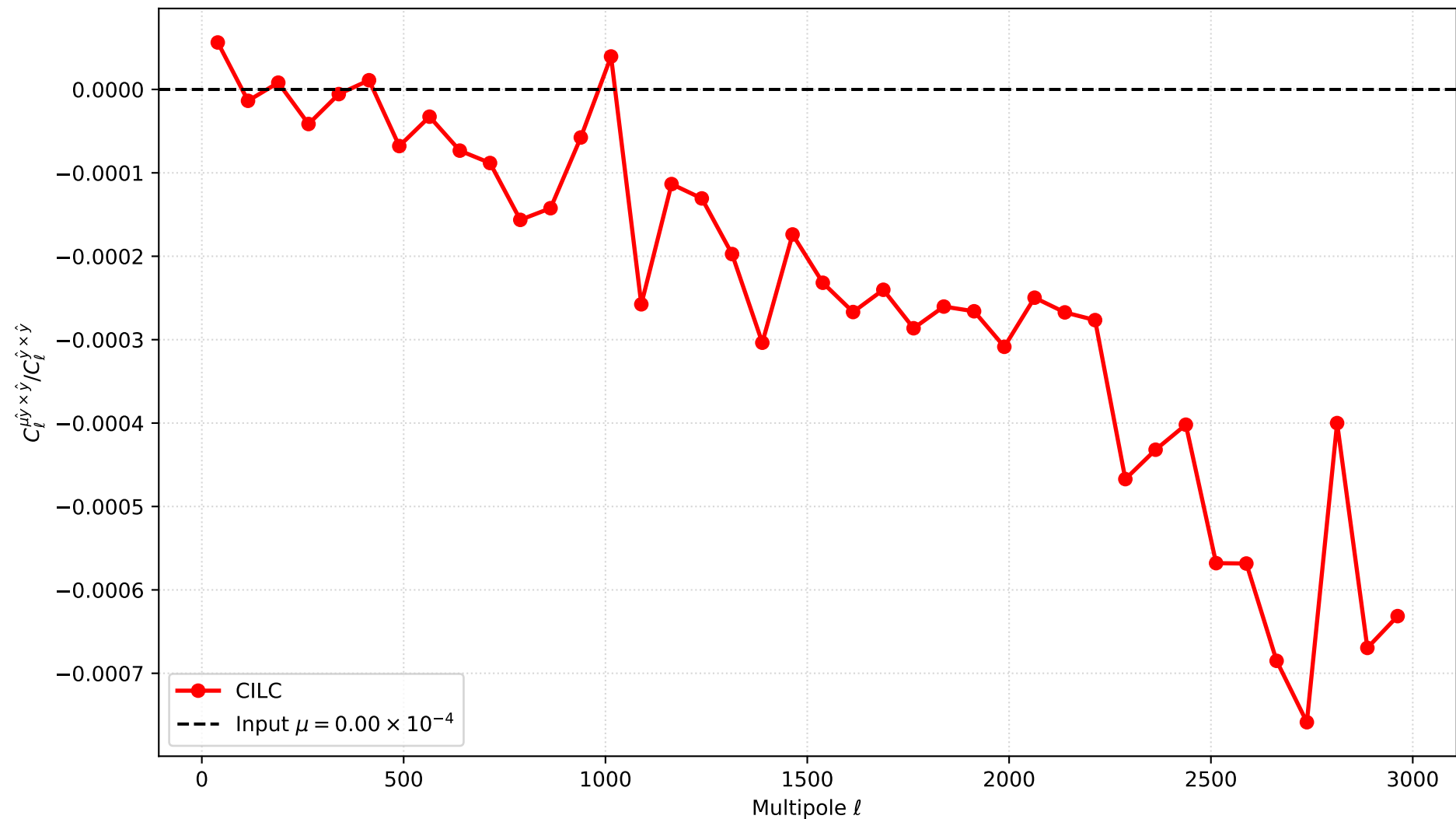
Binned spectral ratio for \mu extraction, \mu = 0\text{e}+00 , base sensitivity = 0.20\ \mu\text{K}\cdot\text{arcmin}
