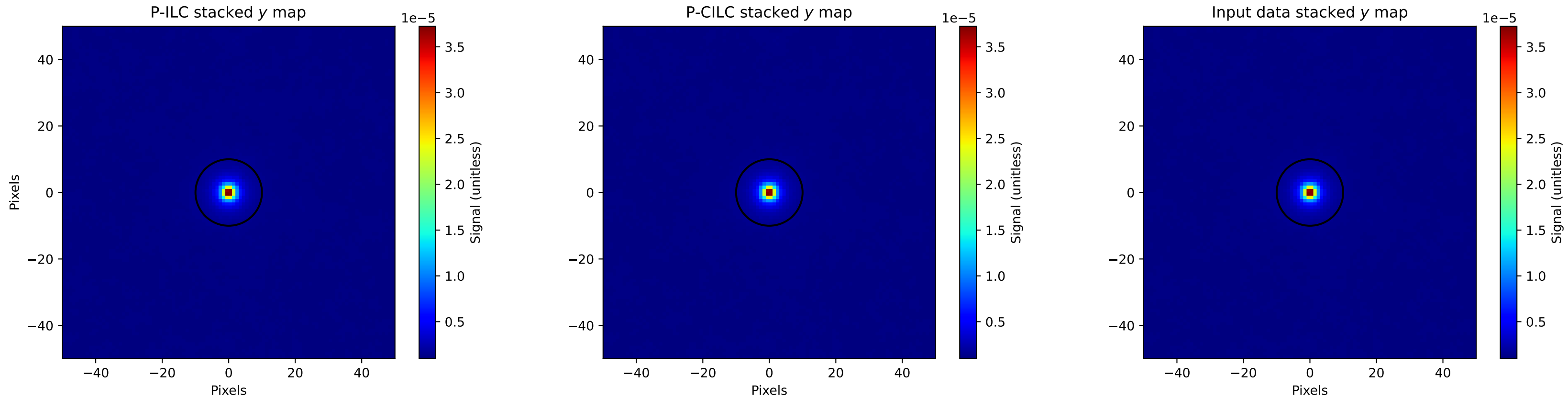
Comparison of y map stacked patches of 1\text{e}+03 brightest clusters, \mu value = 0\text{e}+00 , base sensitivity = 0.20\ \mu\text{K}\cdot\text{arcmin} , r = 10\text{p}
