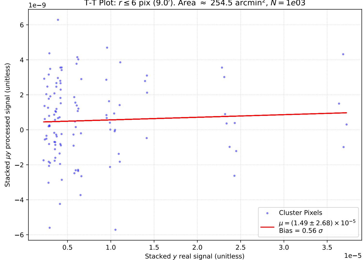
T-T Plot: r \leq 6 pix (9.0'). Area \approx 254.5 arcmin 2 , N = 1e03
