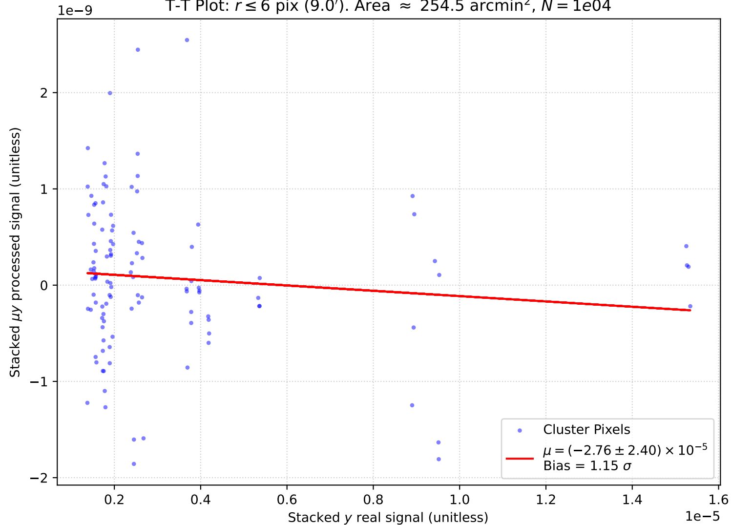
T-T Plot: r \leq 6 pix (9.0'). Area \approx 254.5 arcmin 2 , N = 1e04
