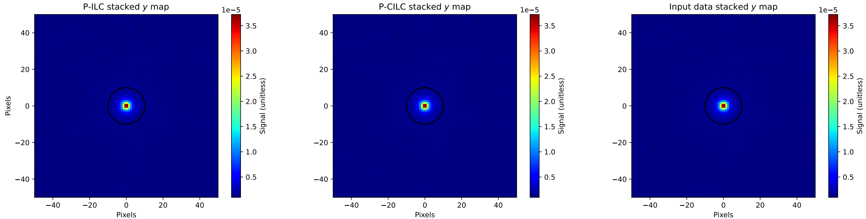
Comparison of y map stacked patches of 1e+03 brightest clusters, \mu value = 2e-04 , r = 10p
