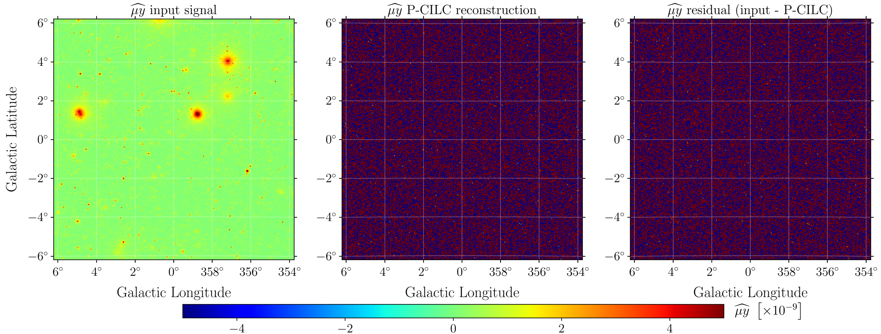
Zoomed input map and P-CILC reconstructed and residual \widehat{\mu y} maps, \mu = 2 \times 10^{-4} , PICO configuration
