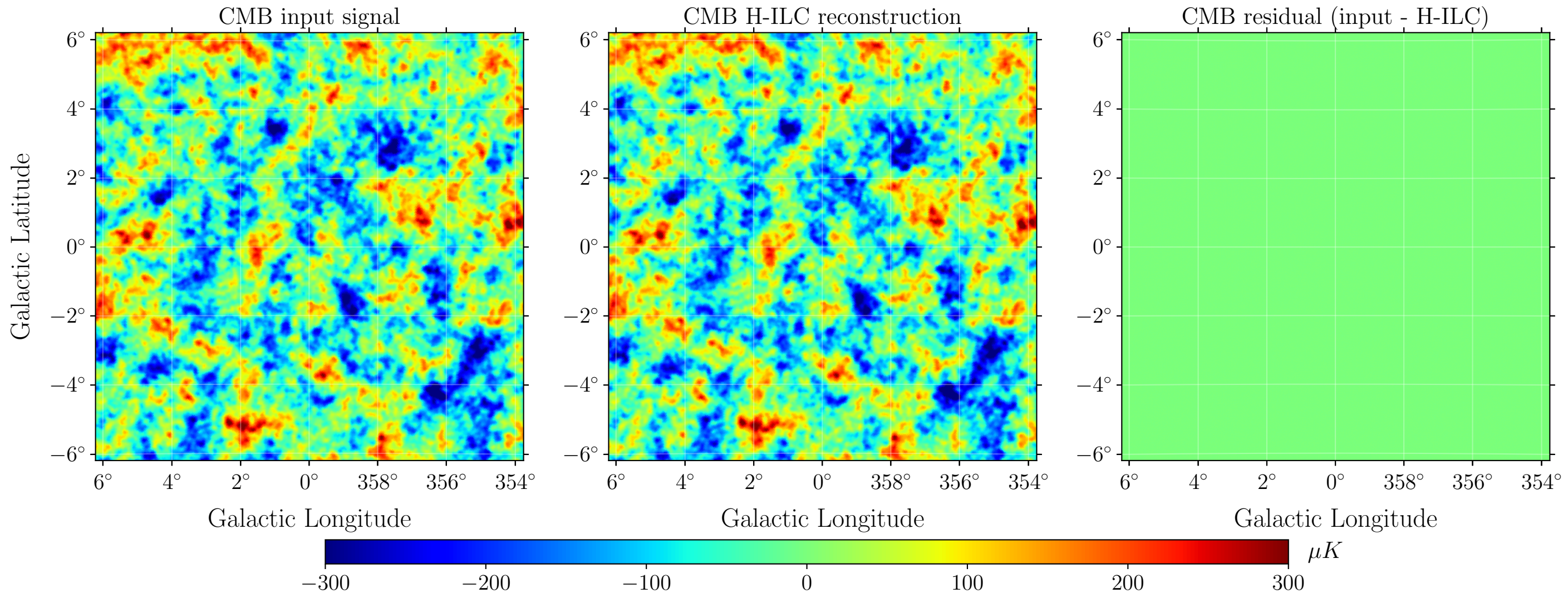
Zoomed input map and H-ILC reconstructed and residual CMB maps, \mu = 2 \times 10^{-4} , PICO configuration
