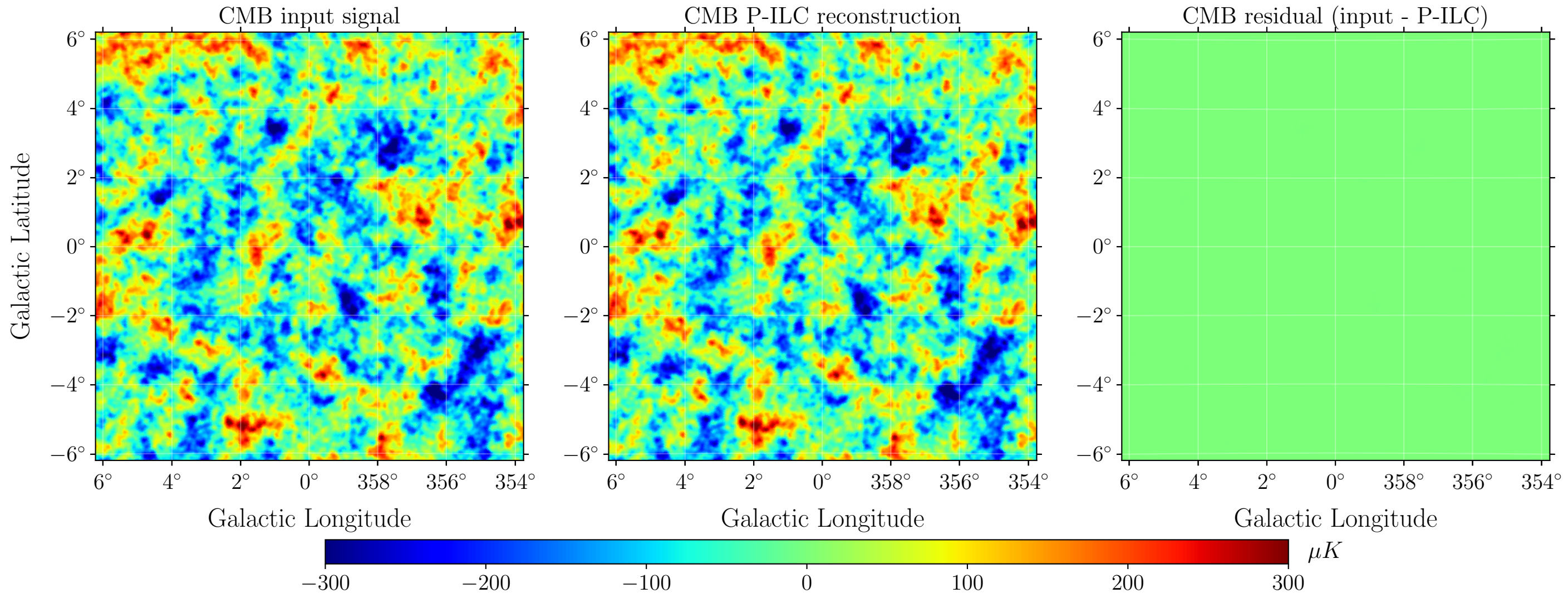
Zoomed input map and P-ILC reconstructed and residual CMB maps, \mu = 2 \times 10^{-4} , PICO configuration
