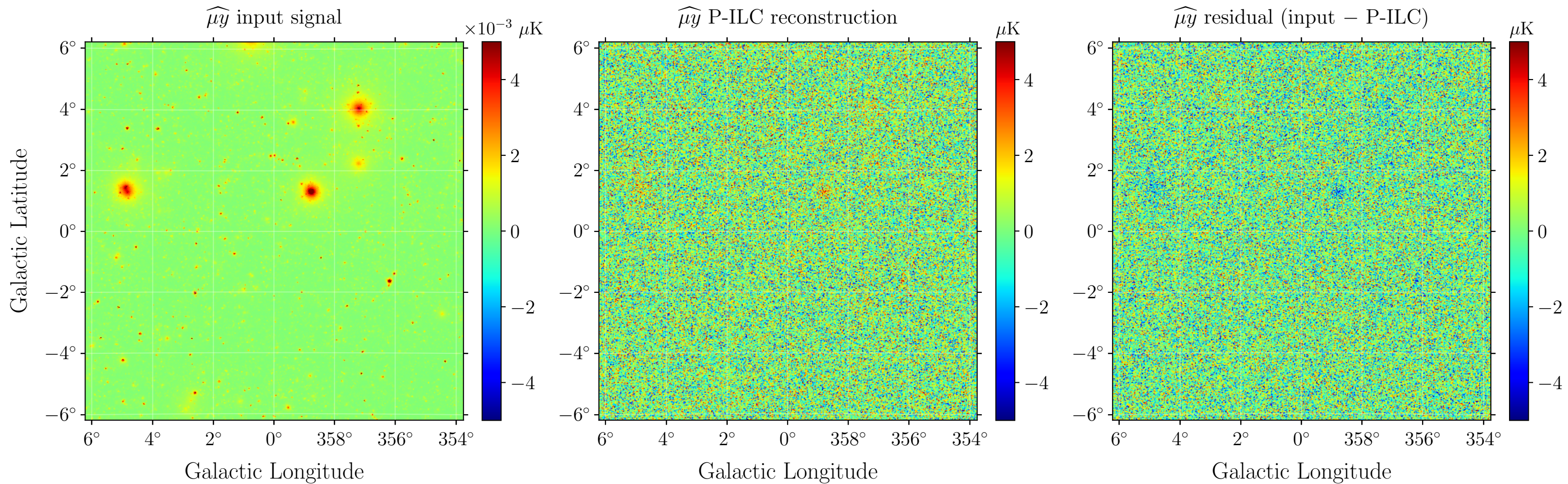
Zoomed input map and P-ILC reconstructed and residual \widehat{\mu y} maps, \mu_{\text{input}} = 2 \times 10^{-4} , PICO configuration
