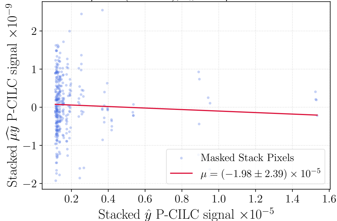
T-T Plot for \mu extraction, N = 10^4 , 200 iterations, CMB-HD-like, \mu = 0 (null test), s_n = 0.2 \mu\text{K}\cdot\text{arcmin}
